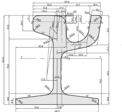
Figuur 2.11 Groove rails; 54G1/54R1 (ArcelorMittal, 2021)
