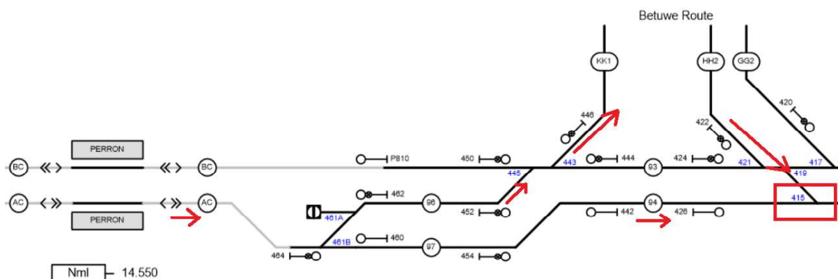
Figuur C.1 Nijmegen Lent – Betuwe Route - Elst
